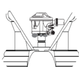
figure 10 Gas cylinder valve/Regulator connection
